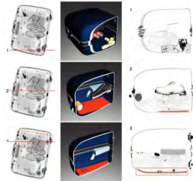
Image Acquisition X-ray imaging
